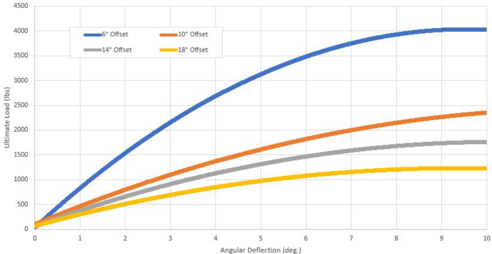
Capacity Chart PSC2060706 and PSC2060717
